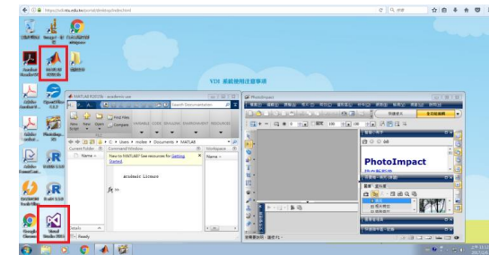
VDI Desktop
